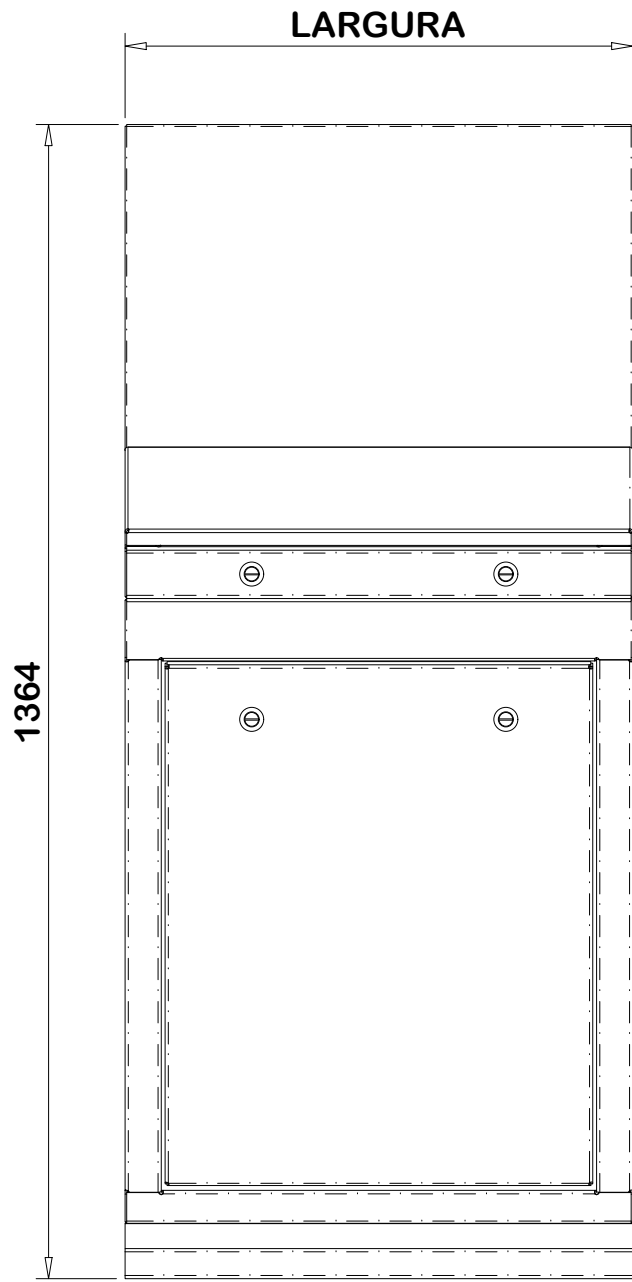
VISTA FRONTAL
