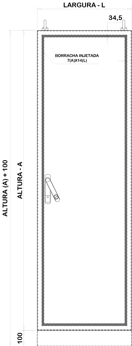
VISTA FRONTAL
